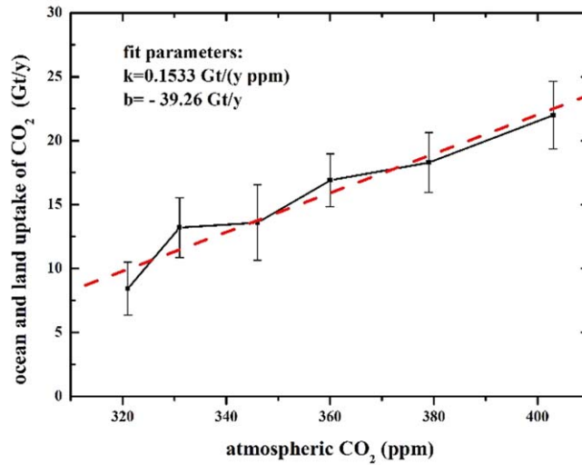
Figure 2. Combined and 10 year averaged annual \text{CO}_2 uptake of oceans and land as a function of atmospheric \text{CO}_2 concentration in the period from 1960 to 2022. The sink data are from [14]. The dashed line denotes a linear fit to the data including uncertainty bars.
