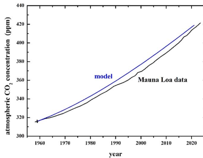
Figure 4. Comparison of Mauna Loa data for atmospheric CO 2 concentration (lower line) with model results (upper line). The model starts with 316 ppm in 1960. Total emissions Q_{\text{tot}} increase linearly from 17 Gt/y in 1960 to 41 Gt/y in 2021.
