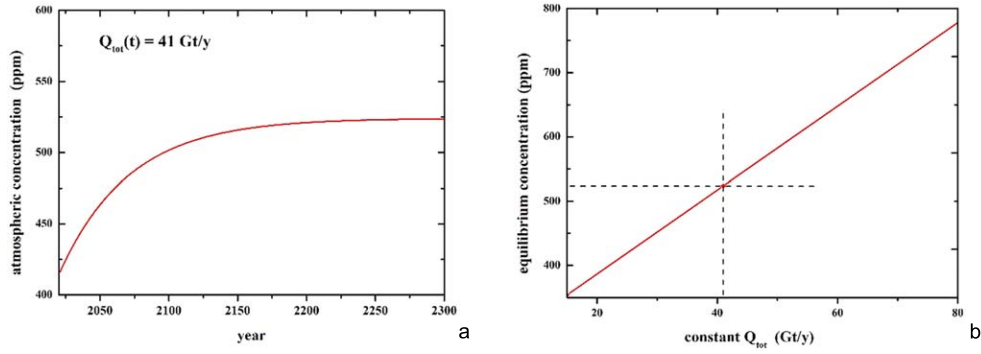
Figure 3. (a) Model result for constant emission rate of 41 Gt/y. The CO 2 concentration in the atmosphere will ultimately reach an equilibrium value of 524 ppm (horizontal line). (b) Change of equilibrium value as function of constant emission rate. Present emission data are indicated by the vertical dashed line and the respective equilibrium value by the horizontal dashed line.
