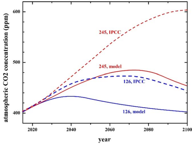
Figure 5. Comparison of IPCC and model \text{CO}_2 concentrations for IPCC scenarios 126 and 245. The last two digits of the scenario characterize the additional radiative forcing, here 2.6 \text{ W m}^{-2} and 4.5 \text{ W m}^{-2} . For emission input data, see figure 6 and text.
