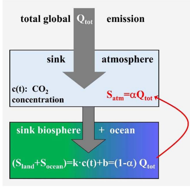
Figure 1. Schematic representation of the model. The total global emission Q_{\text{tot}} into the atmosphere enters the atmosphere. A fraction (1-\alpha) thereof ends up in the biosphere and ocean combined. The remaining part S_{\text{atm}} stays in the atmosphere. Details, see text.
